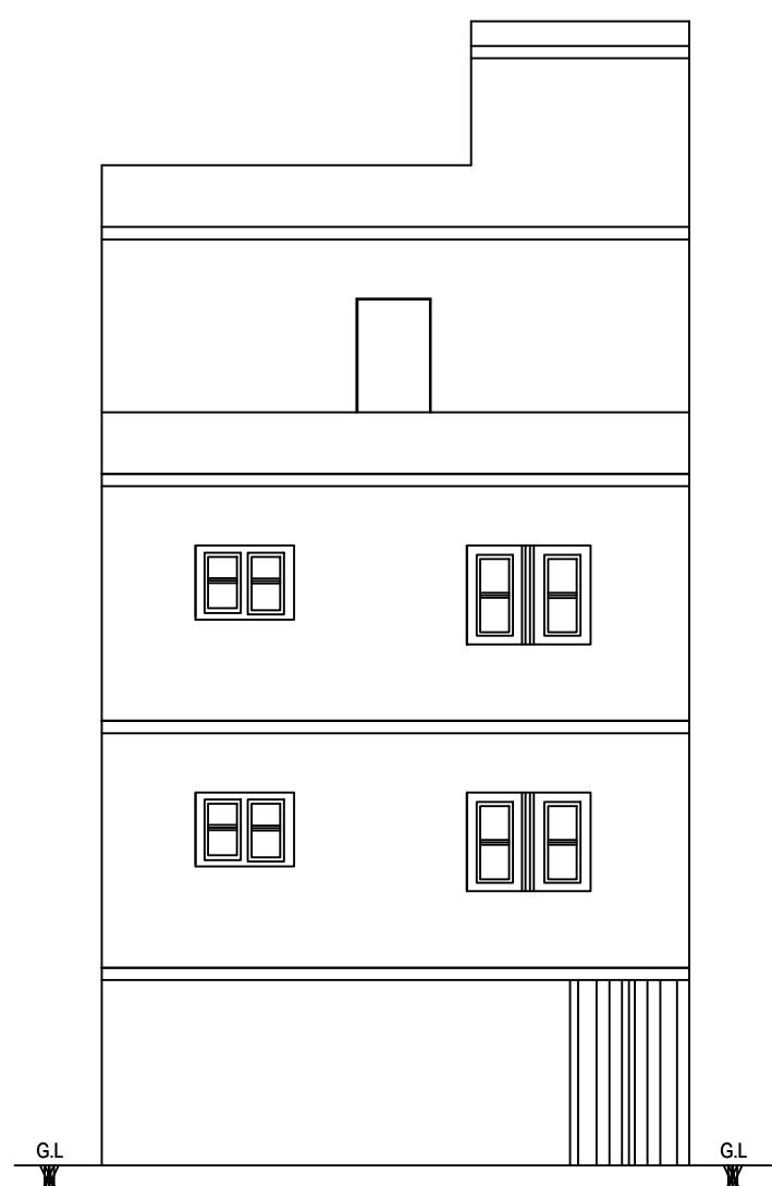
FRONT ELEVATION
